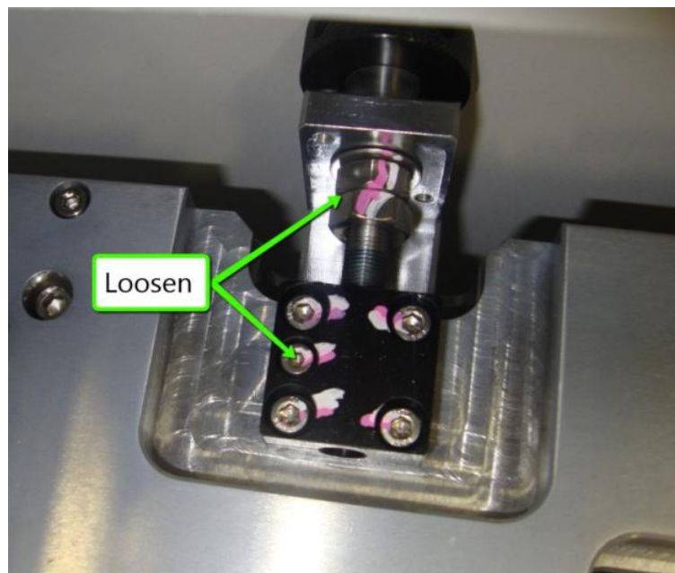
Figure 10 Tube Adjustment Knob
