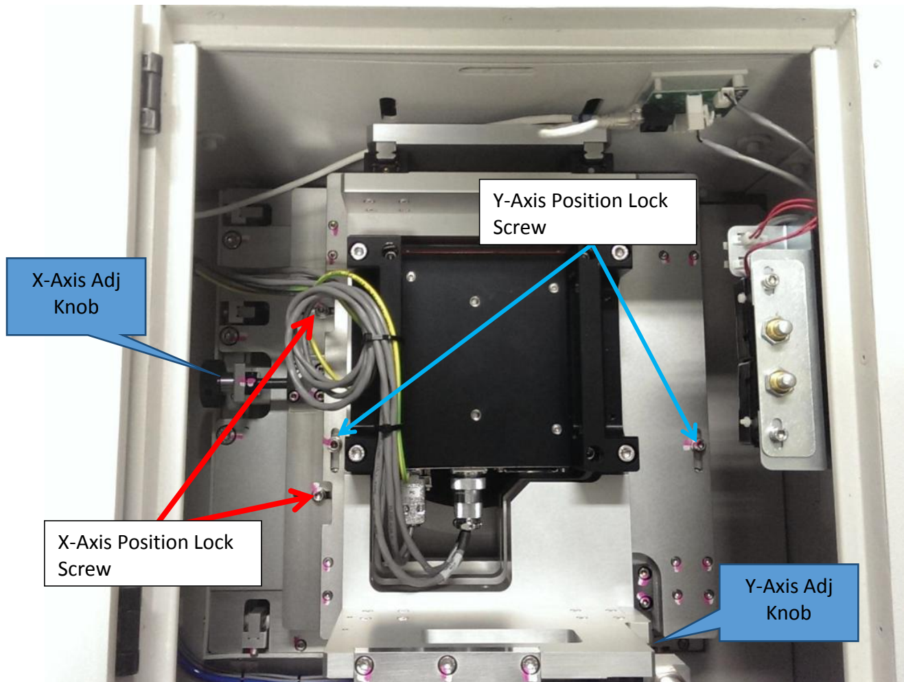
Figure 9 X ray Tube assembly
