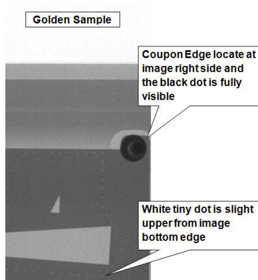
Figure 7 X ray spot [GOLDEN SAMPLE]
